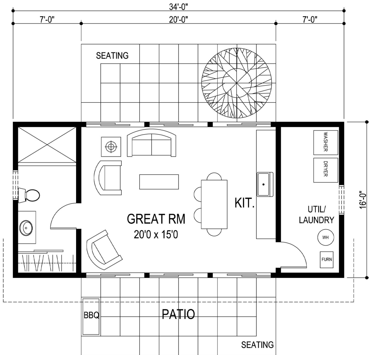
FLOOR PLAN 544 s.f.
